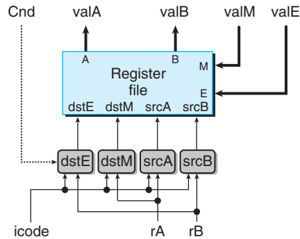
Figure 4.28 SEQ decode and write-back stage. The instruction fields are decoded to generate register identifiers for four addresses (two read and two write) used by the register file. The values read from the register file become the signals valA and valB . The two write-back values valE and valM serve as the data for the writes.
